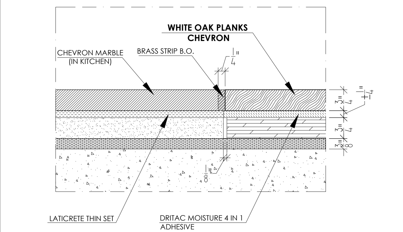
5 WOOD FLOOR TO STONE FLOOR - TYPICAL DETAIL 6" = 1'-0"
