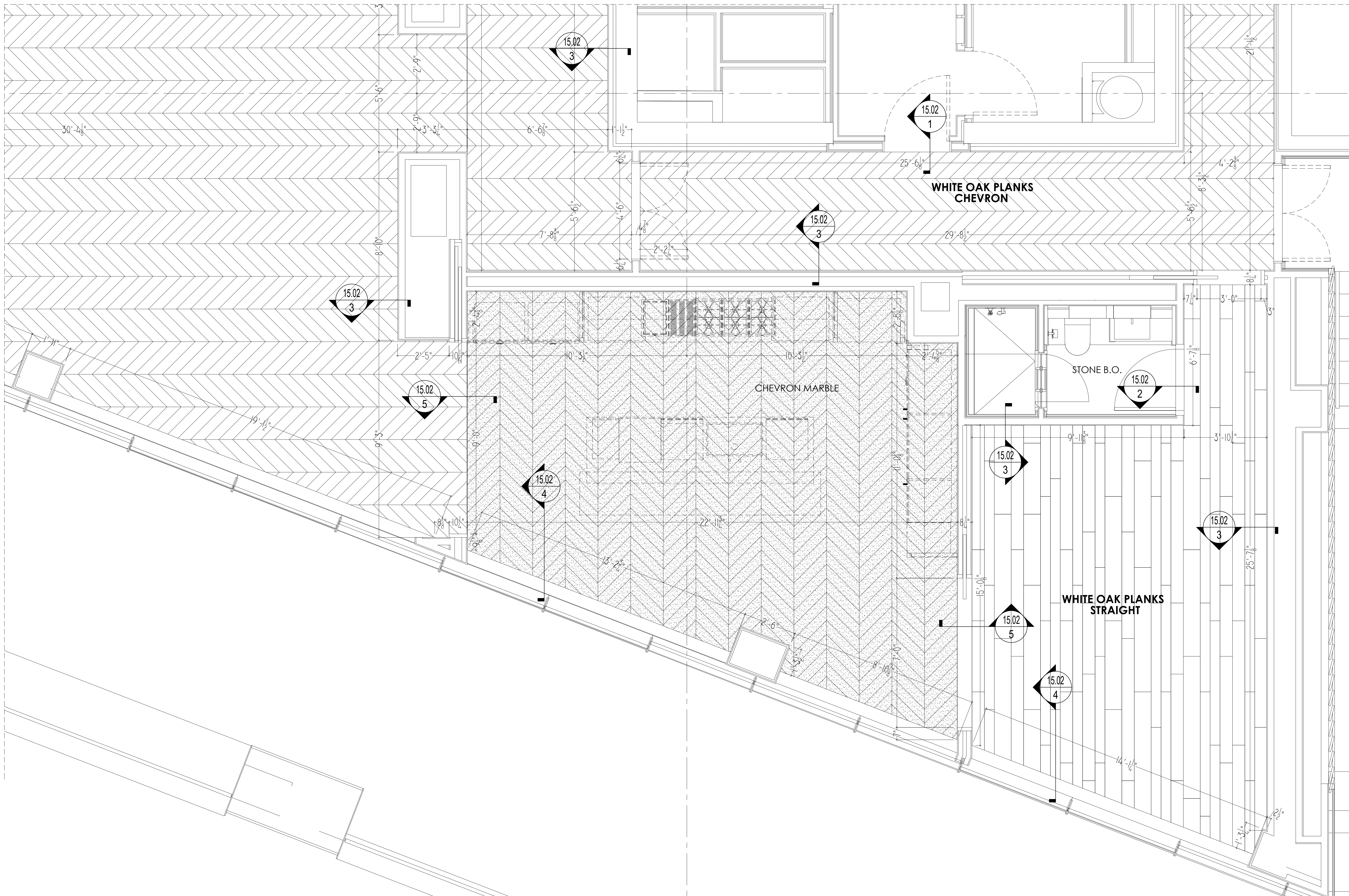
25TH FLOOR - UNIT #E-5-PH-X PLAN PART F
