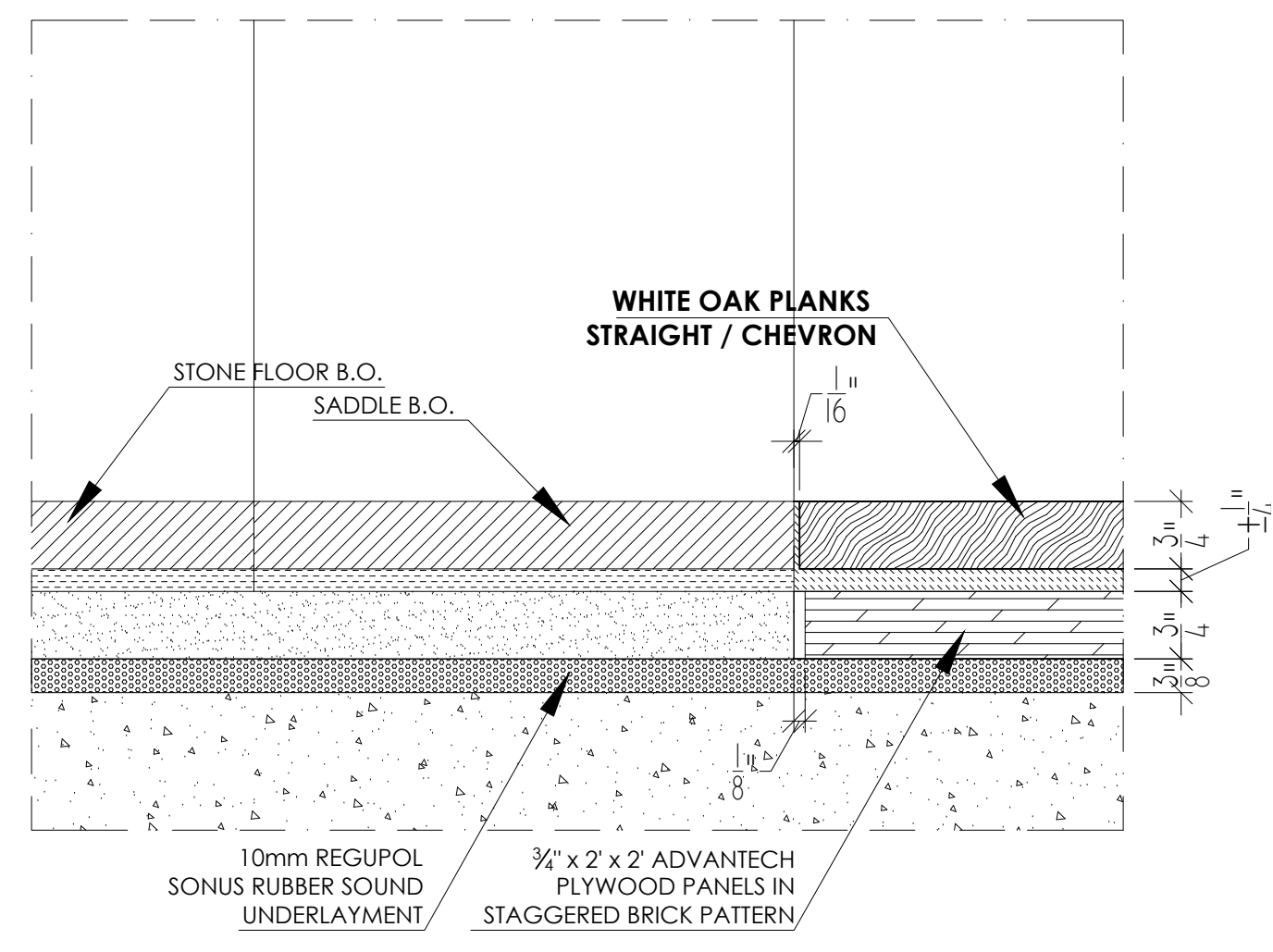
2 TYP SADDLE TO BATHROOM 6" = 1'-0"
