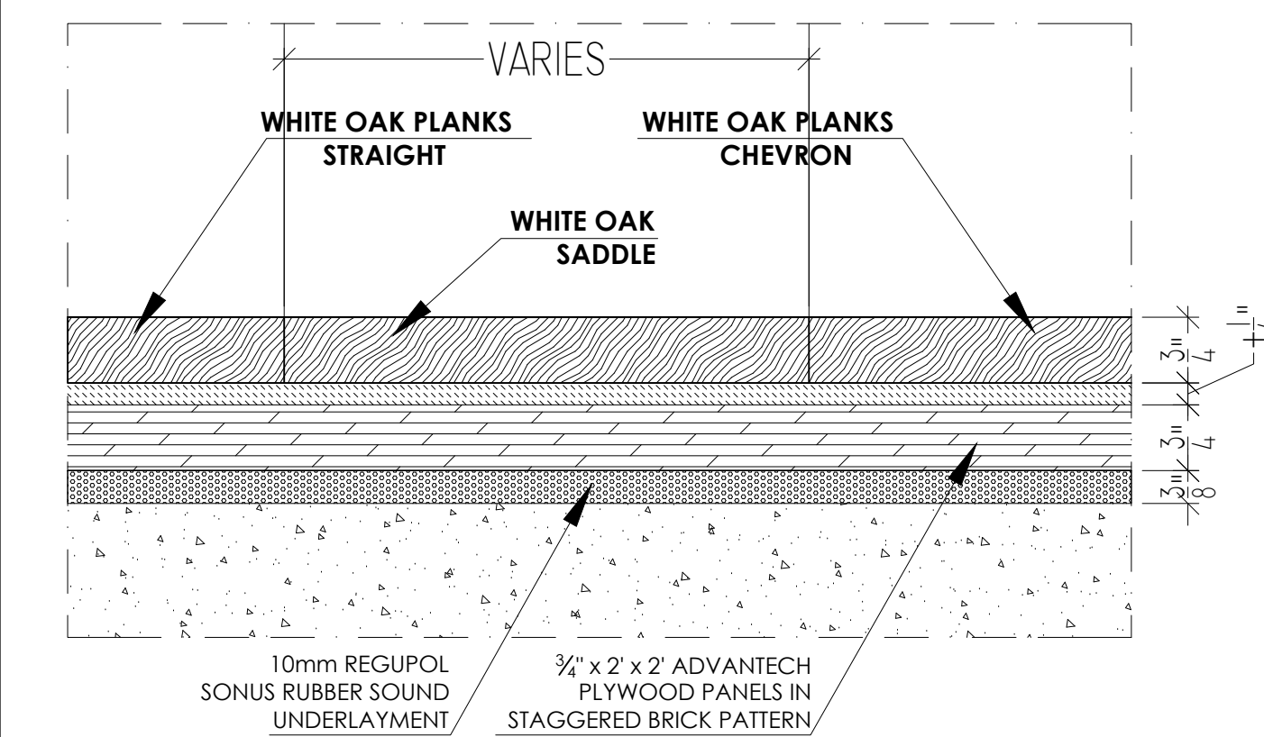
6 WOOD FLOOR TO WOOD FLOOR - TYPICAL DETAIL 6" = 1'-0"
