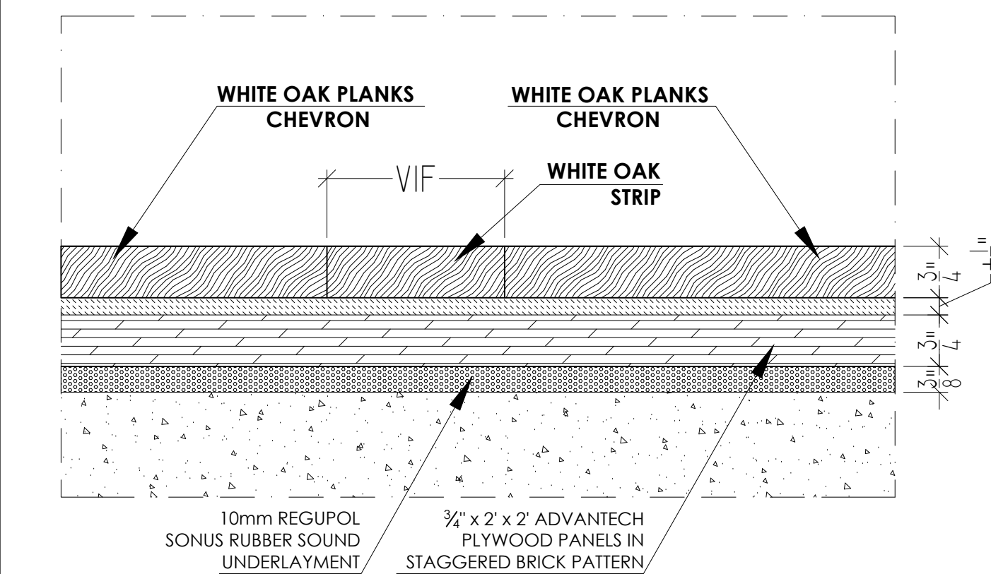
7 WOOD FLOOR TO WOOD FLOOR - TYPICAL DETAIL 6" = 1'-0"
