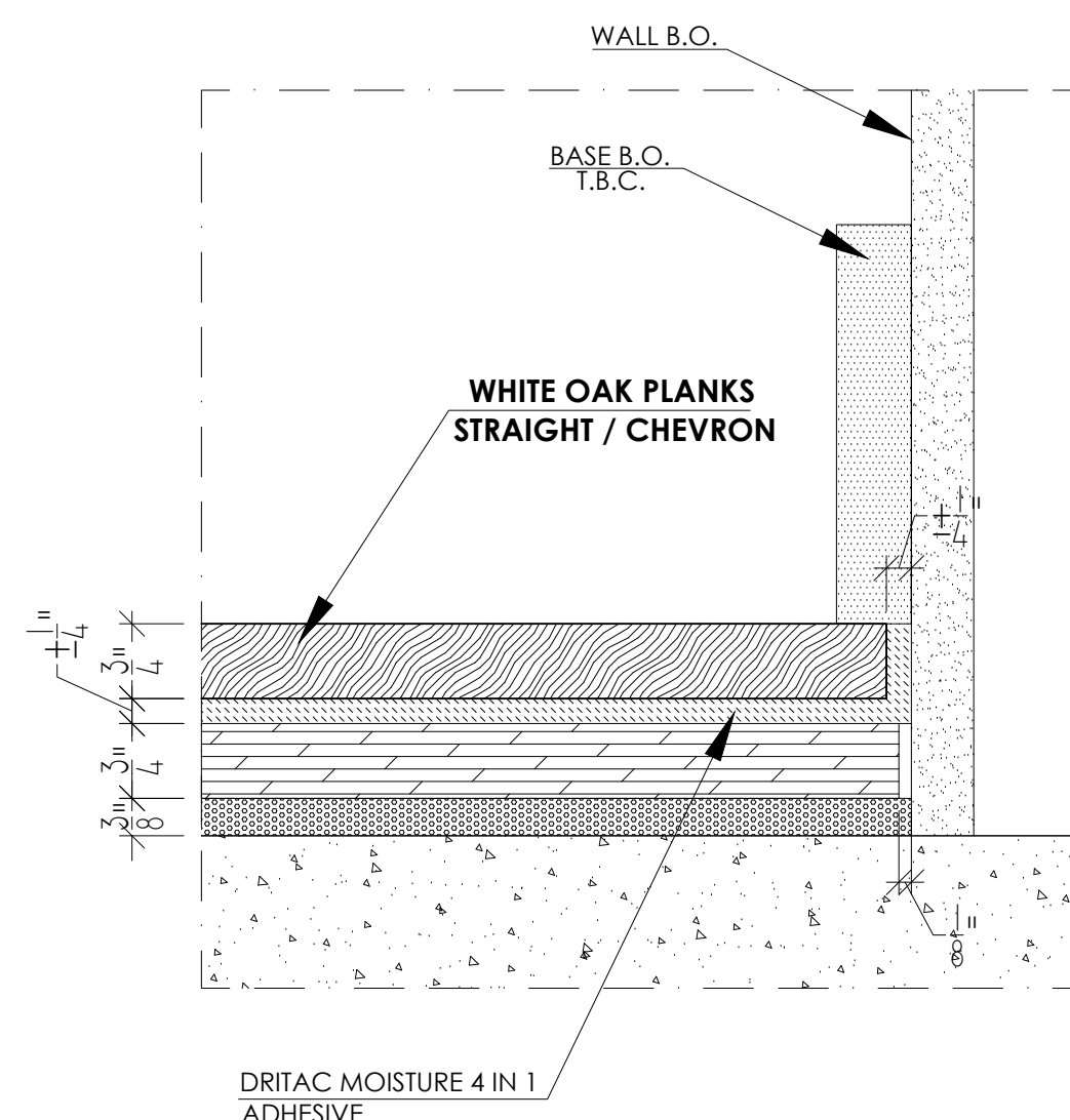
3 TYP BASE DETAIL 6" = 1'-0"
