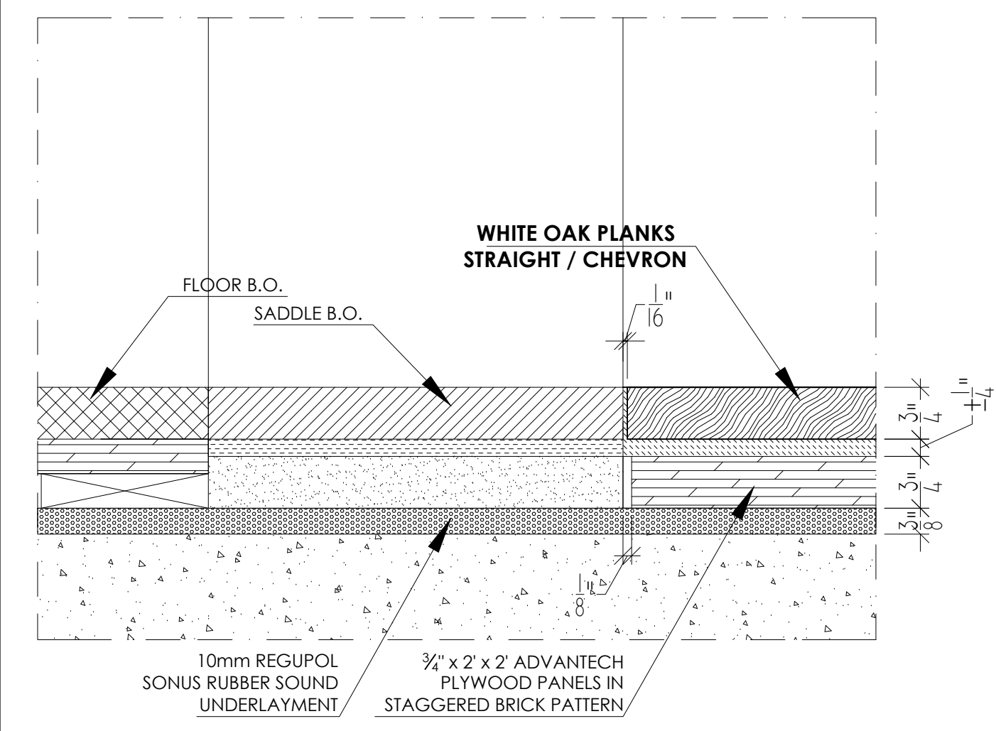
1 TYP ENTRY SADDLE DETAIL 6" = 1'-0"
