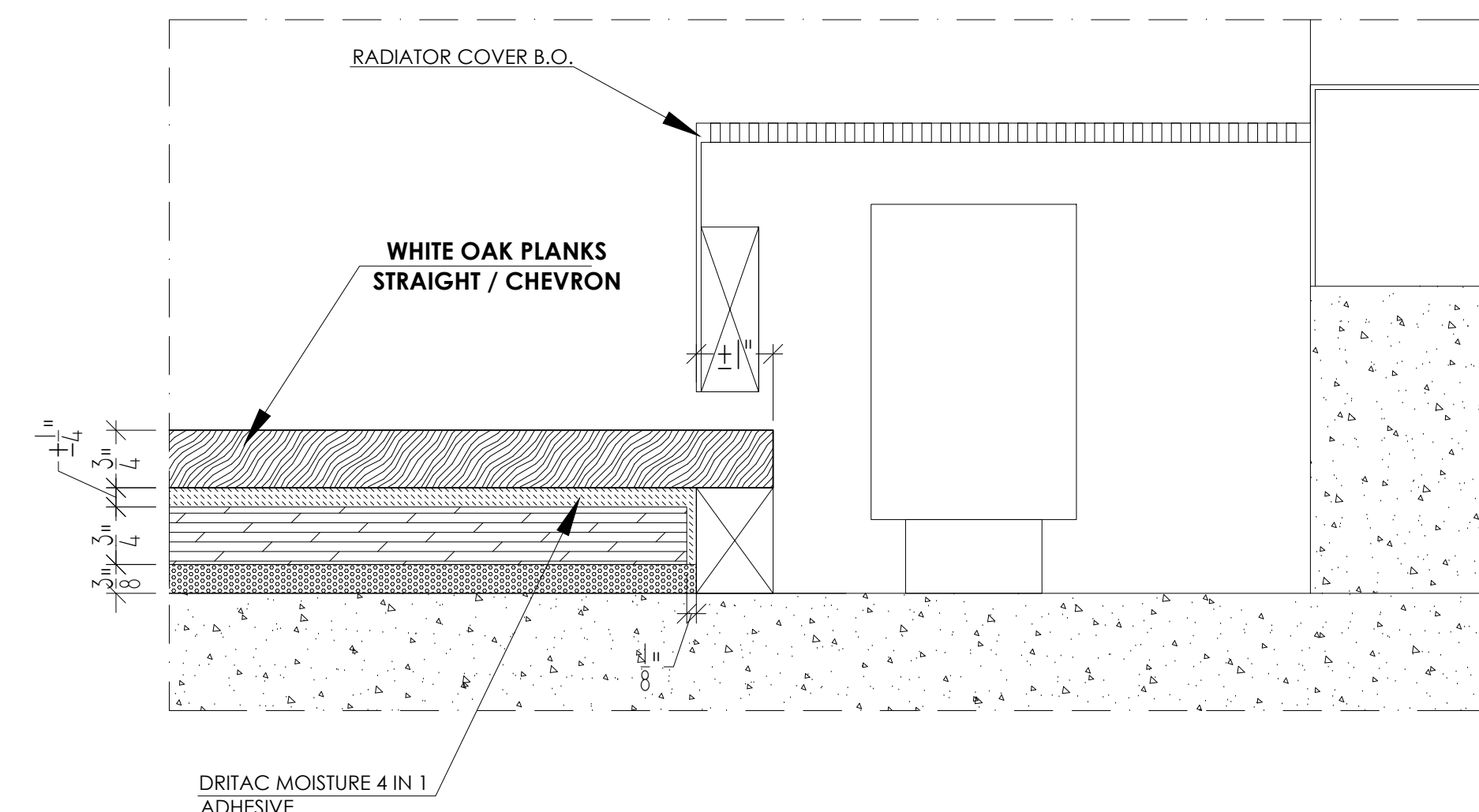
4 WINDOW SILL DETAIL 6" = 1'-0"
