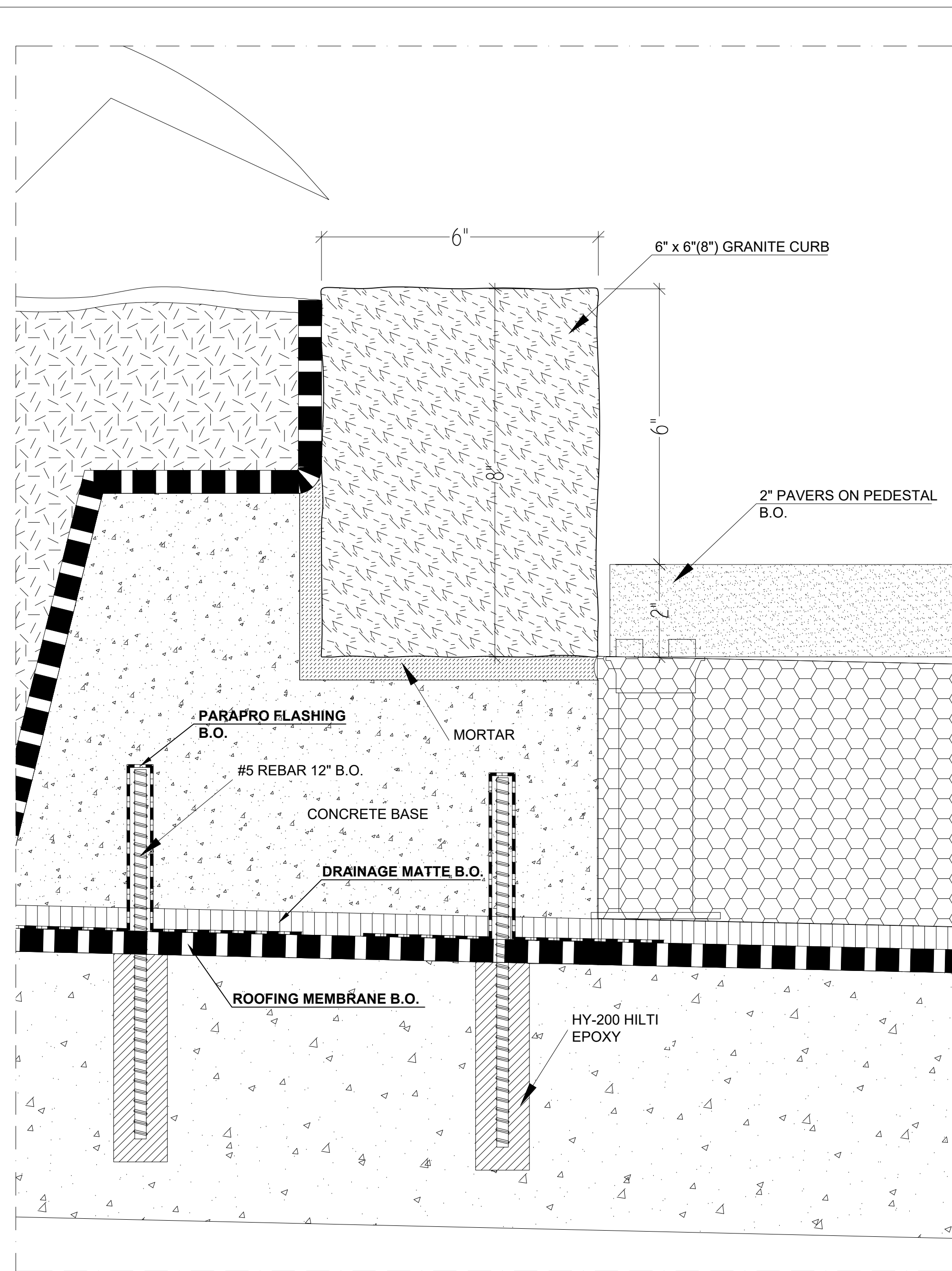
5 GRANITE CURB 6" HEIGHT - DETAIL 6" = 1'-0"
