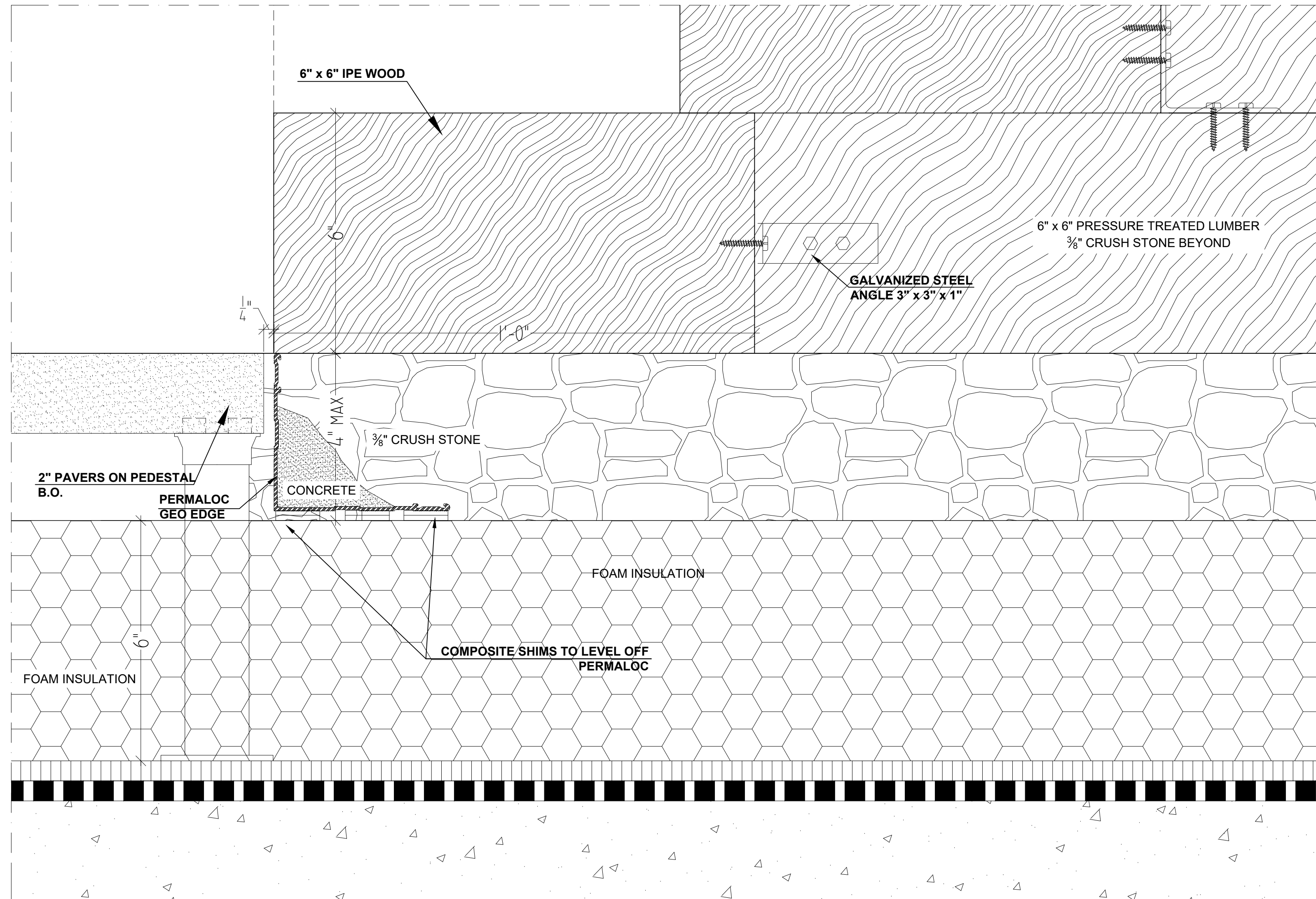
7 TURF MOUND - DETAIL 6" = 1'-0"
