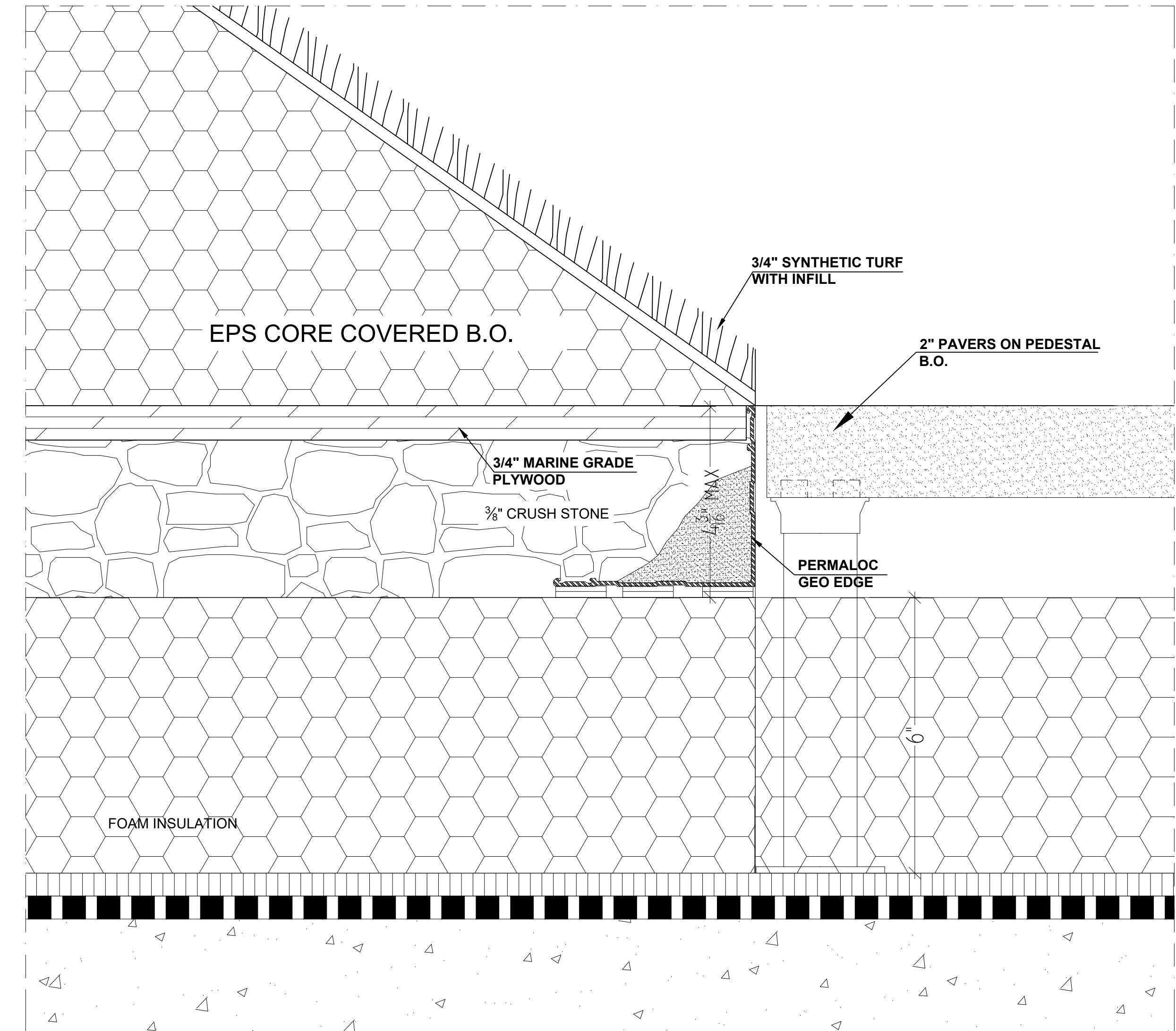
8 TURF MOUND - DETAIL 6" = 1'-0"
