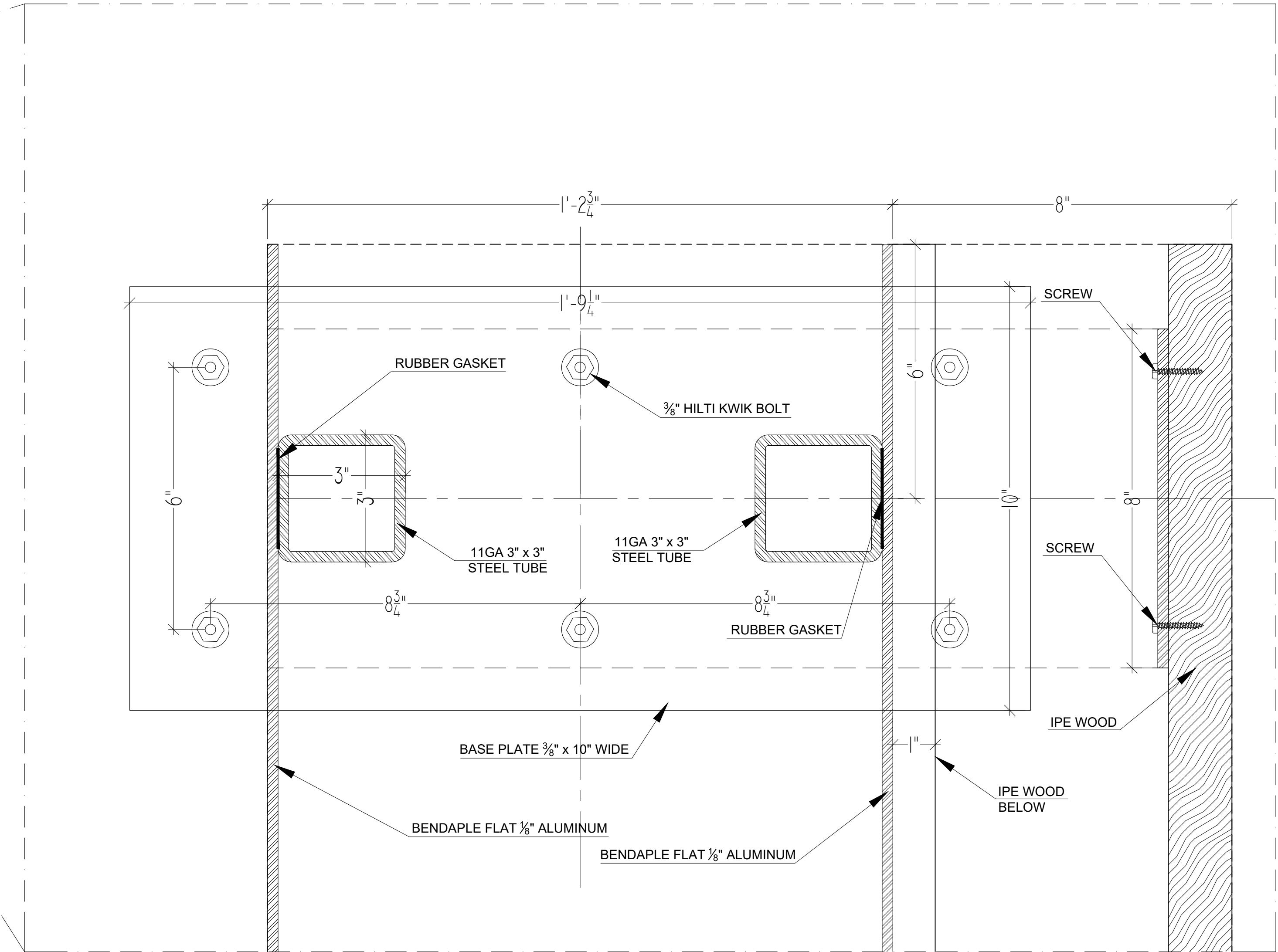
2 IPE BENCH SECTION B DETAIL 6" = 1'-0"
