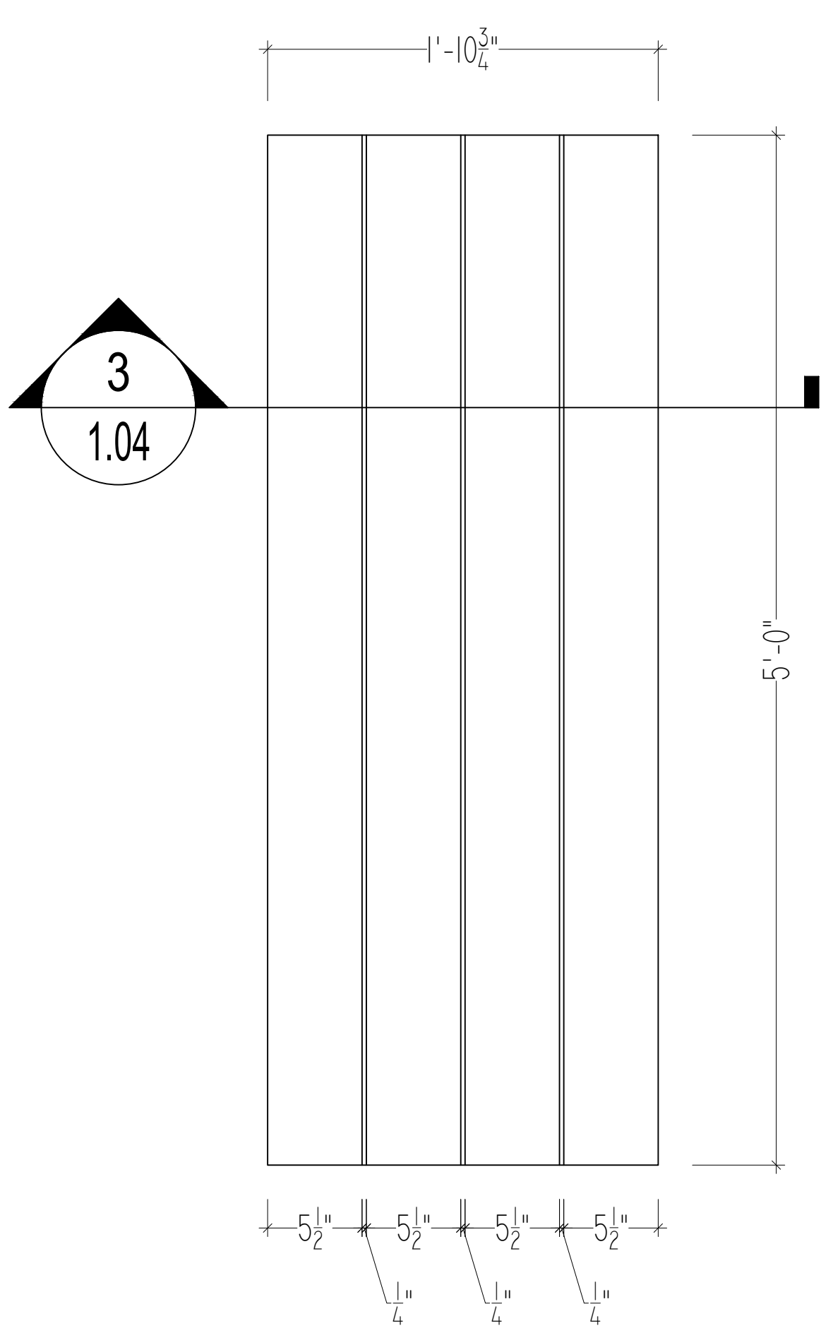
IPE BENCH - PLAN
