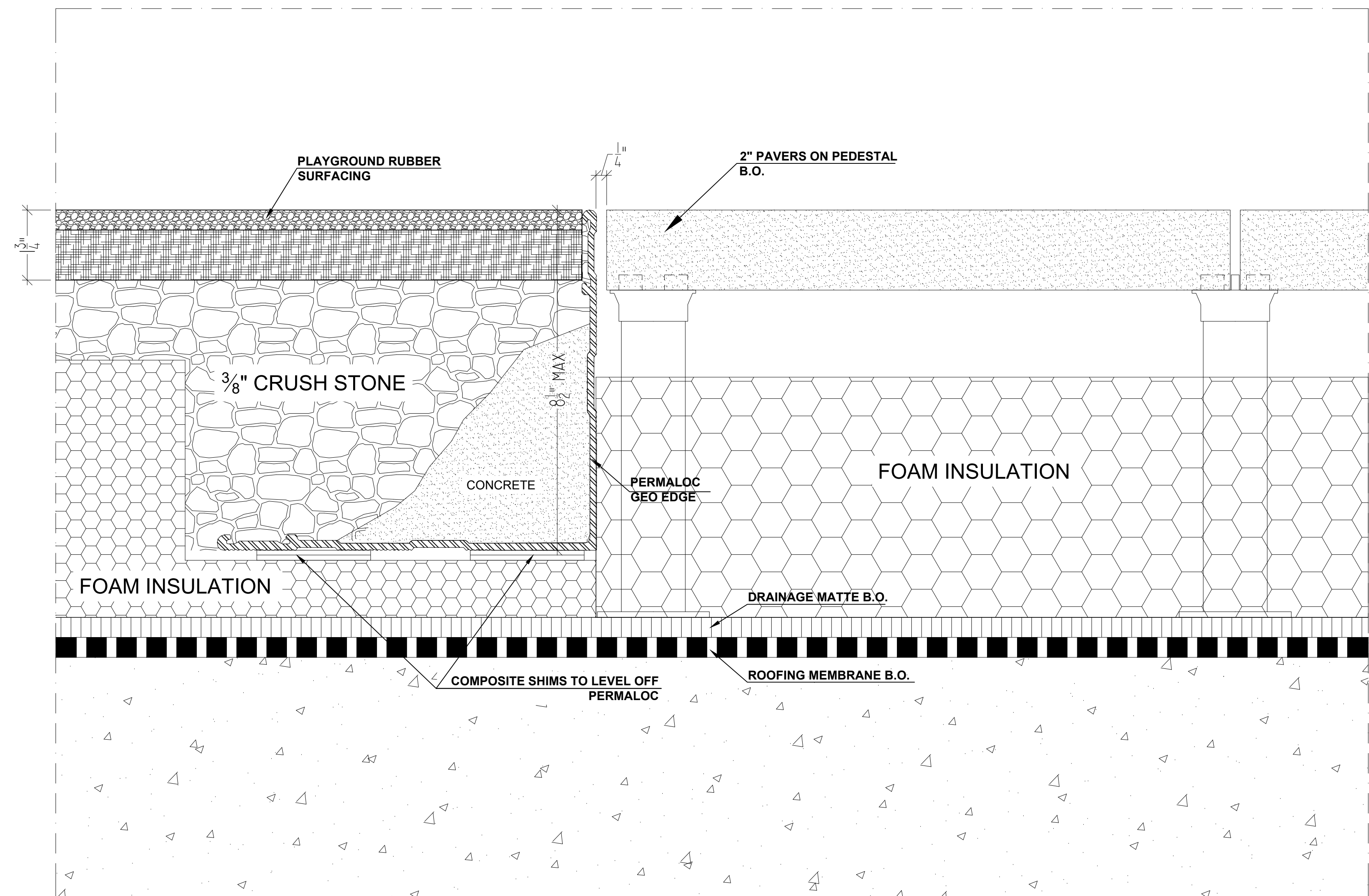
11 PLAYGROUND SURFACING - DETAIL 6" = 1'-0"
