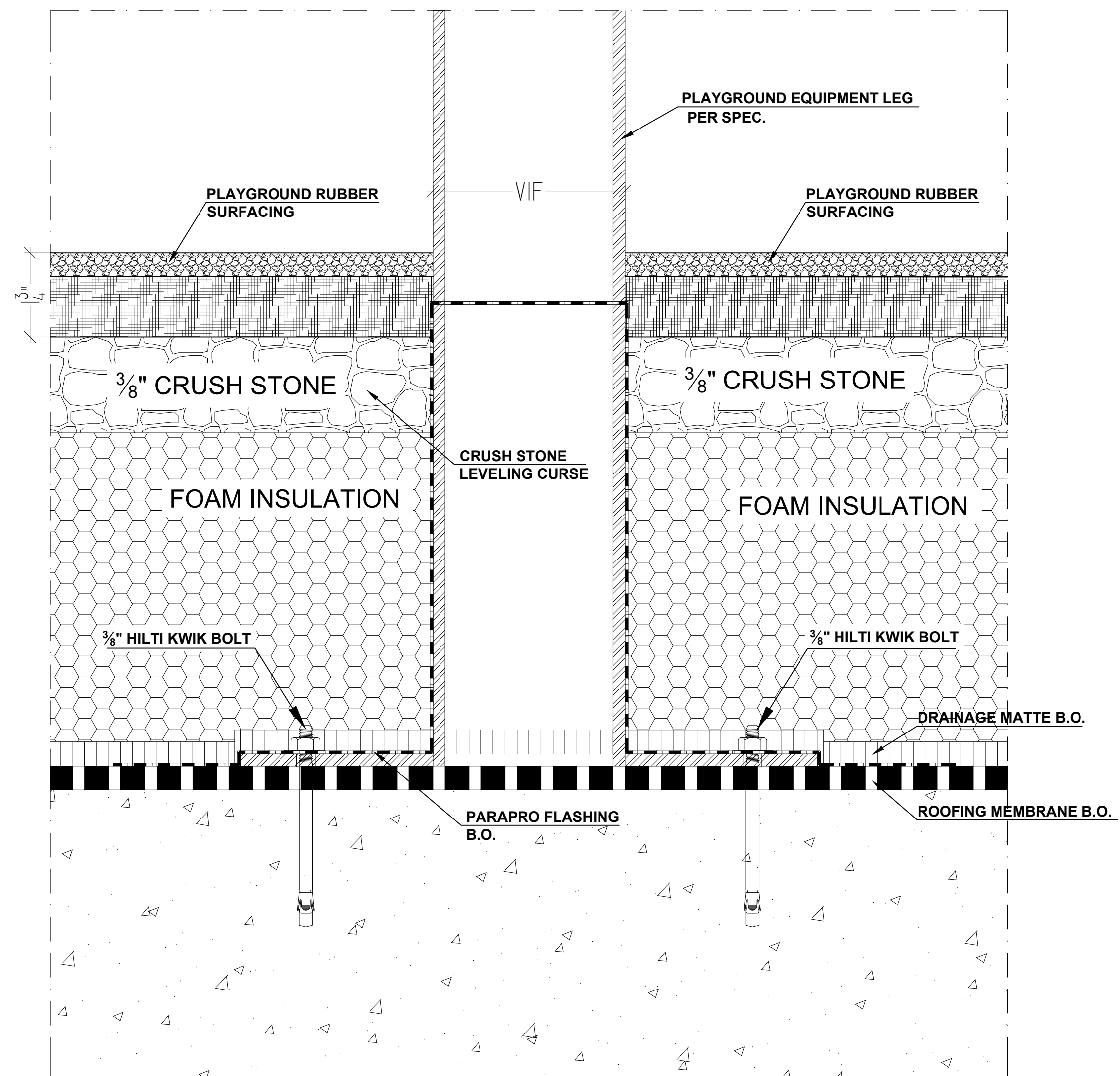
10 PLAYGROUND SURFACING - DETAIL 6" = 1'-0"
