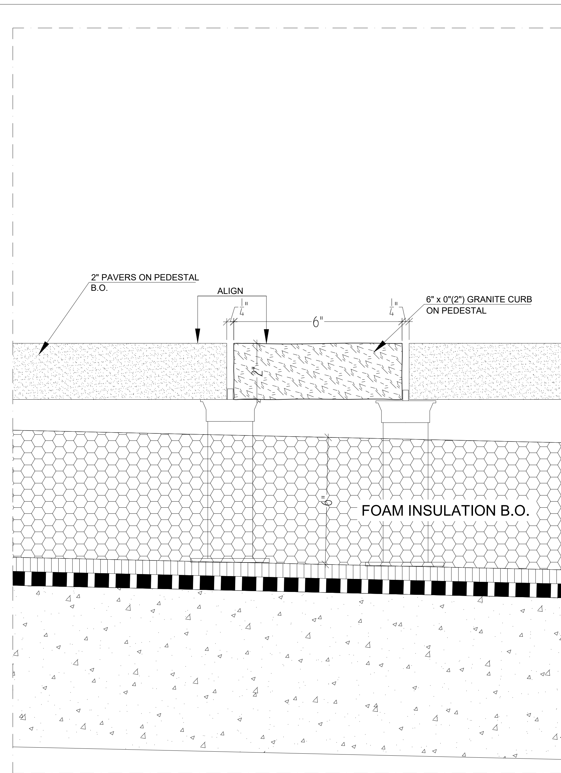
6 GRANITE CURB 0" HEIGHT - DETAIL 6" = 1'-0"
