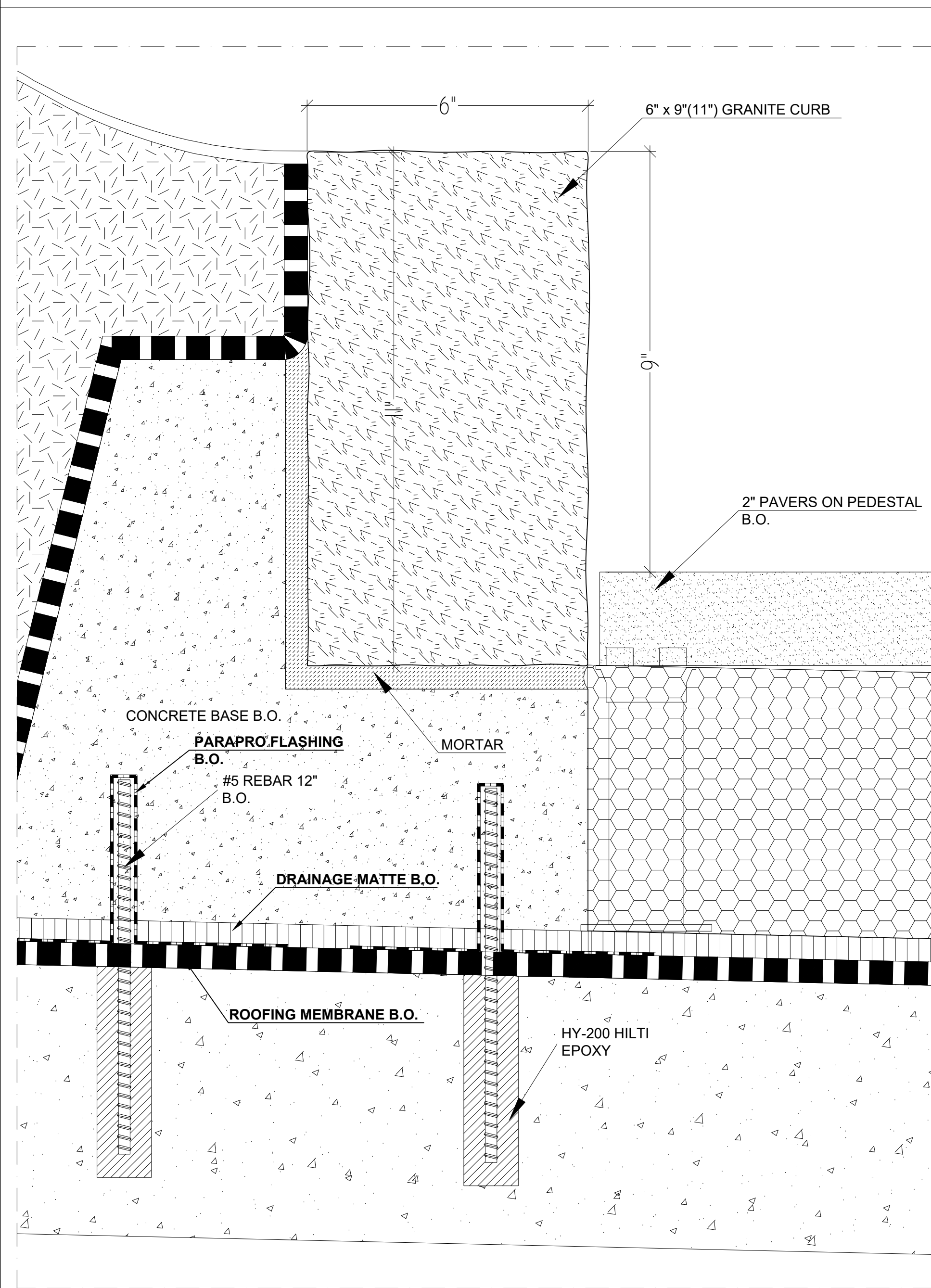
4 GRANITE CURB 9" HEIGHT - DETAIL 6" = 1'-0"
