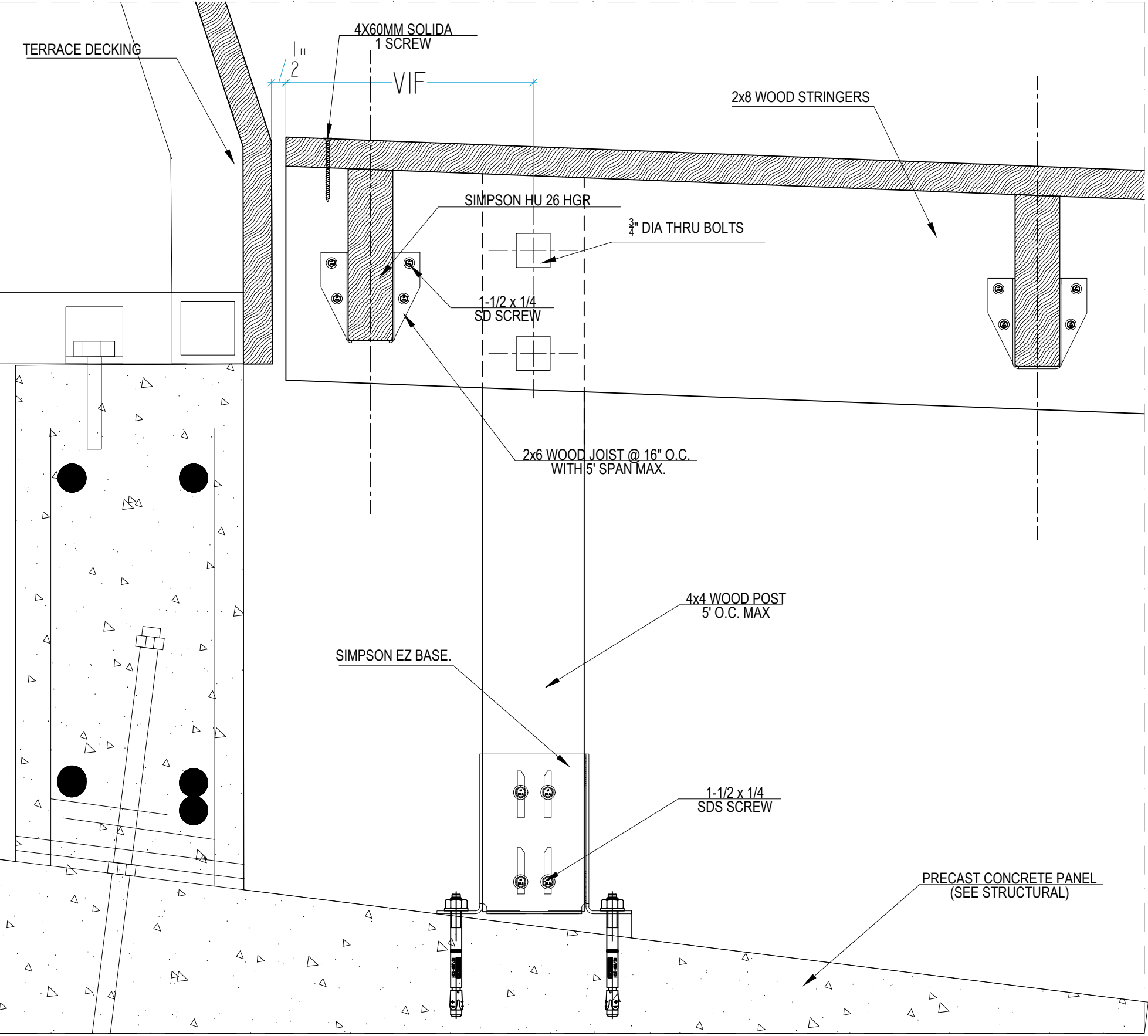
08 WOOD DECKING ON STRUCTURE TO TERRACE 3" = 1'-0"
