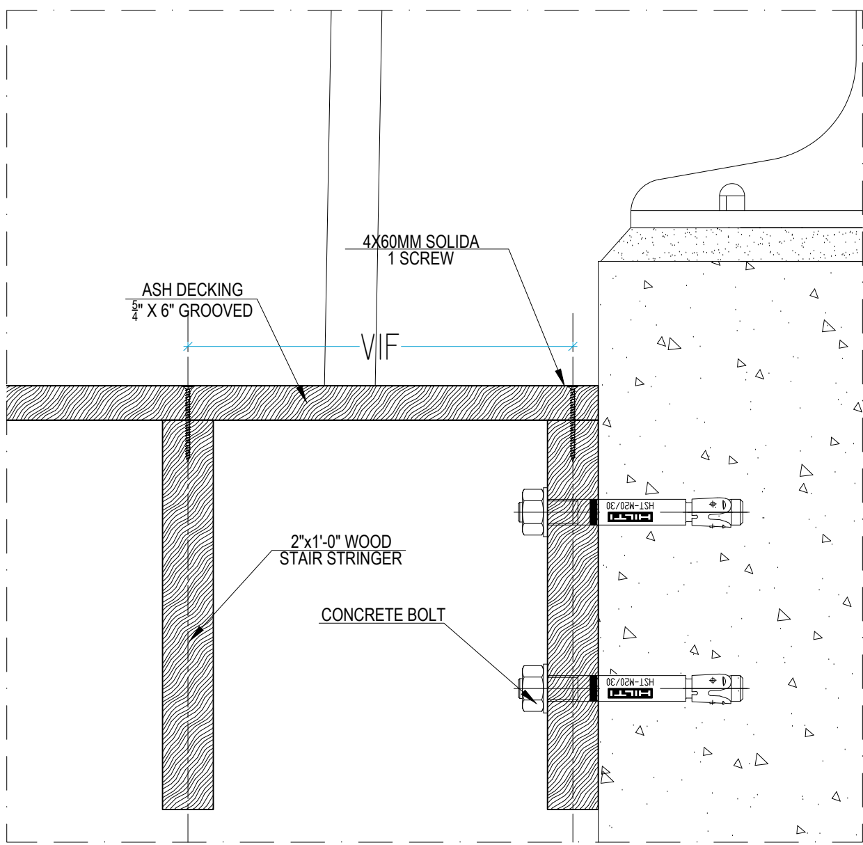
28 WOOD STAIR TO CURB 3" = 1'-0"
