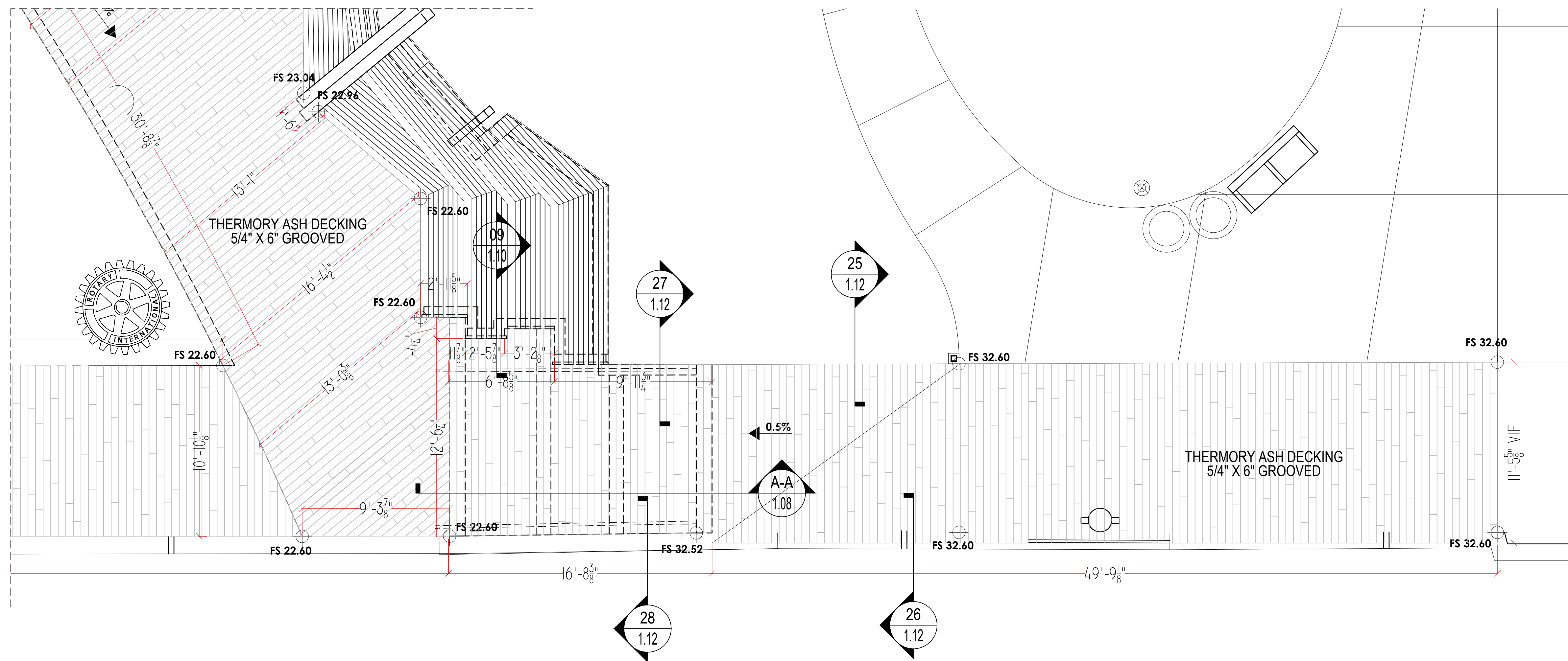
WOOD DECKING - PLAN J
