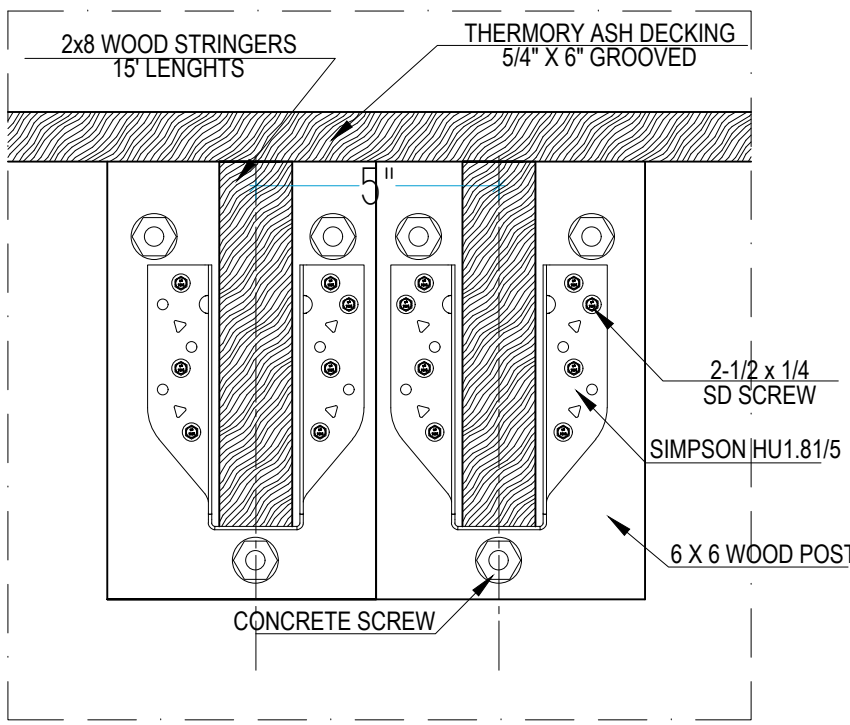
21 TYPICAL SPAN CONNECTION 3" = 1'-0"
