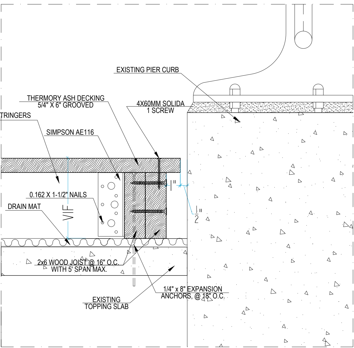
30 DIRECT MOUNT DECKING 3" = 1'-0"
