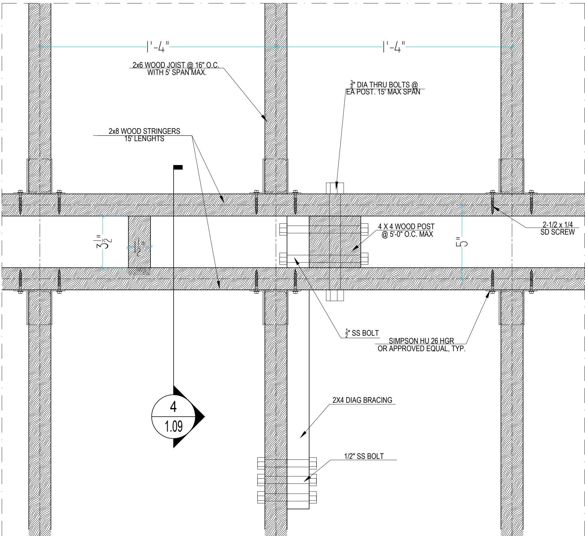
02 TYPICAL SPAN & JOIST CONNECTION 4X4 POST
