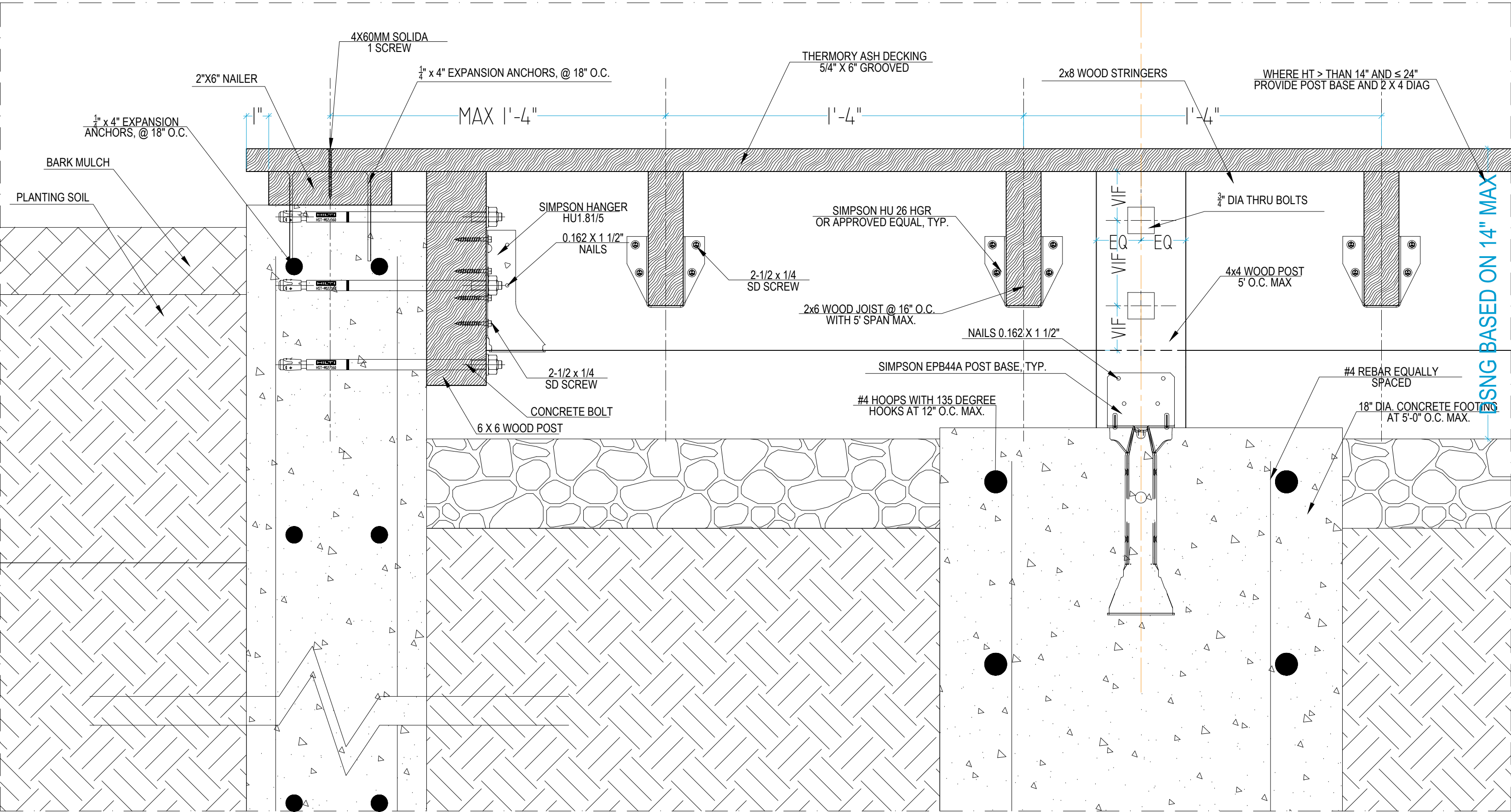
06 CONC. HEADER AT DECKING ON GRADE 3" = 1'-0"
