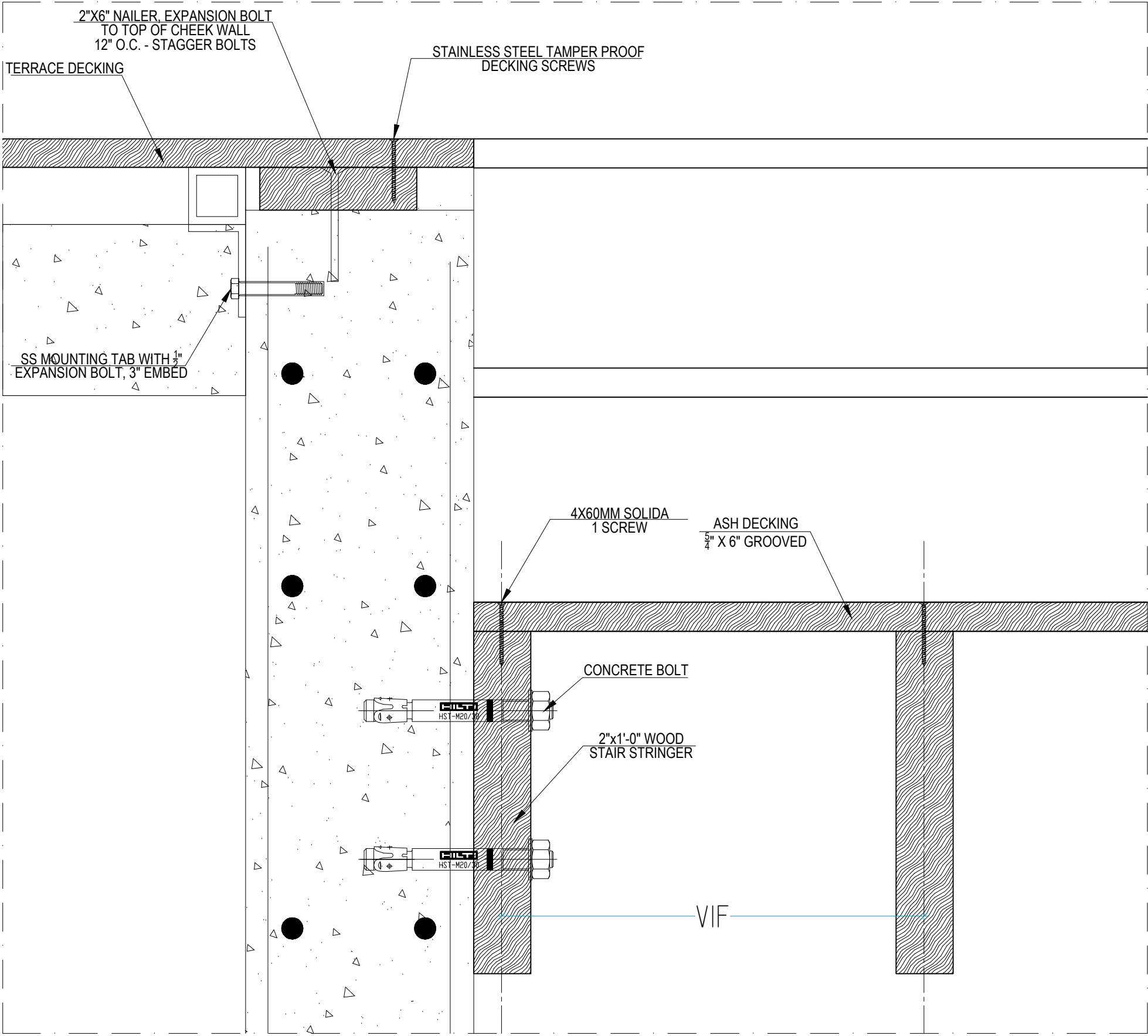
09 WOOD TERRACE CHEEK WALL AT STAIR 3" = 1'-0"
