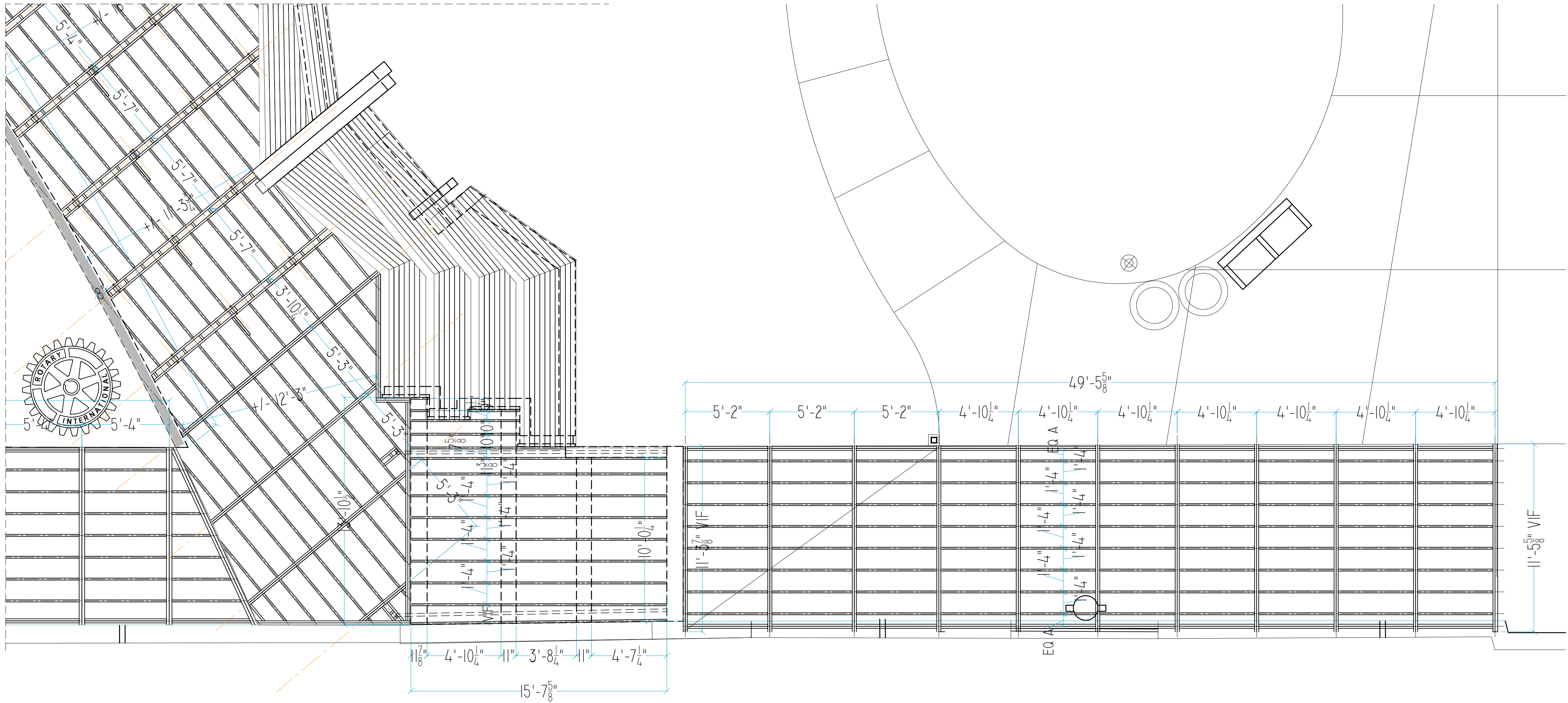
WOOD JOIST & STRINGER - PLAN E
