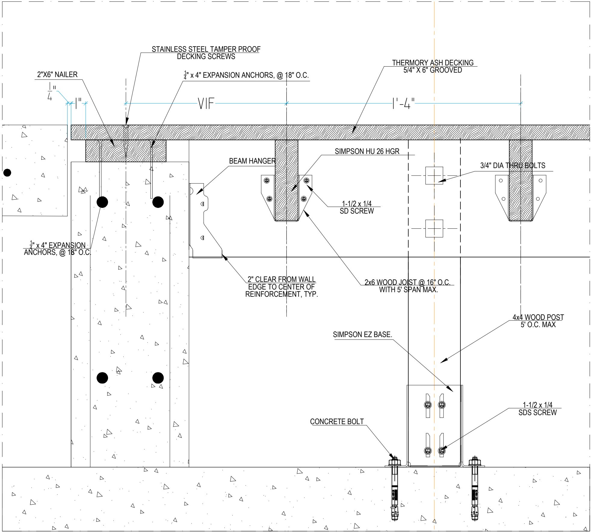
13 CONC. HEADER AT DECKING ON STRUCTURE 3" = 1'-0"
