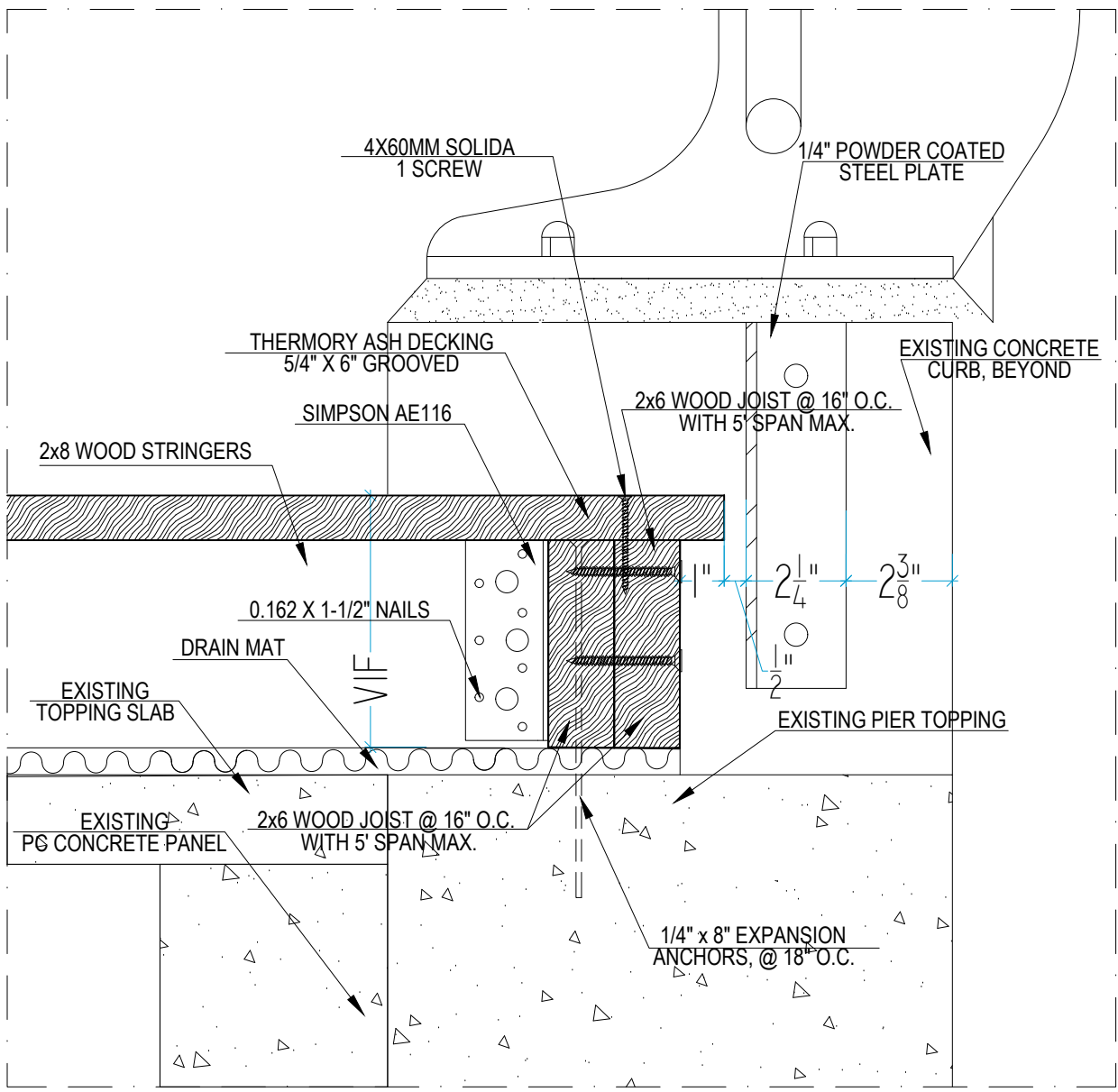
26 DRAINAGE INFILL PANEL 3" = 1'-0"
