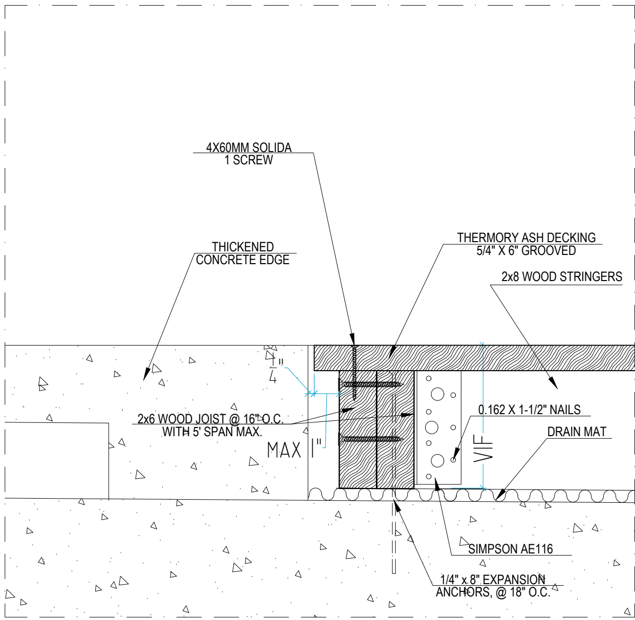
25 CONS. HEADER ON STRUCTURE AT DECKING 3" = 1'-0"
