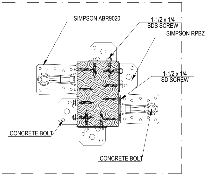
20 WOOD POST DETAIL 3" = 1'-0"
