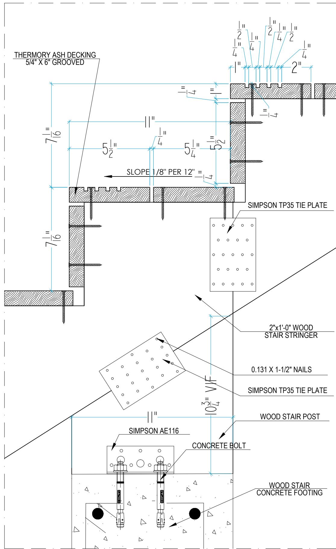
15 STAIR DETAIL 3" = 1'-0"
