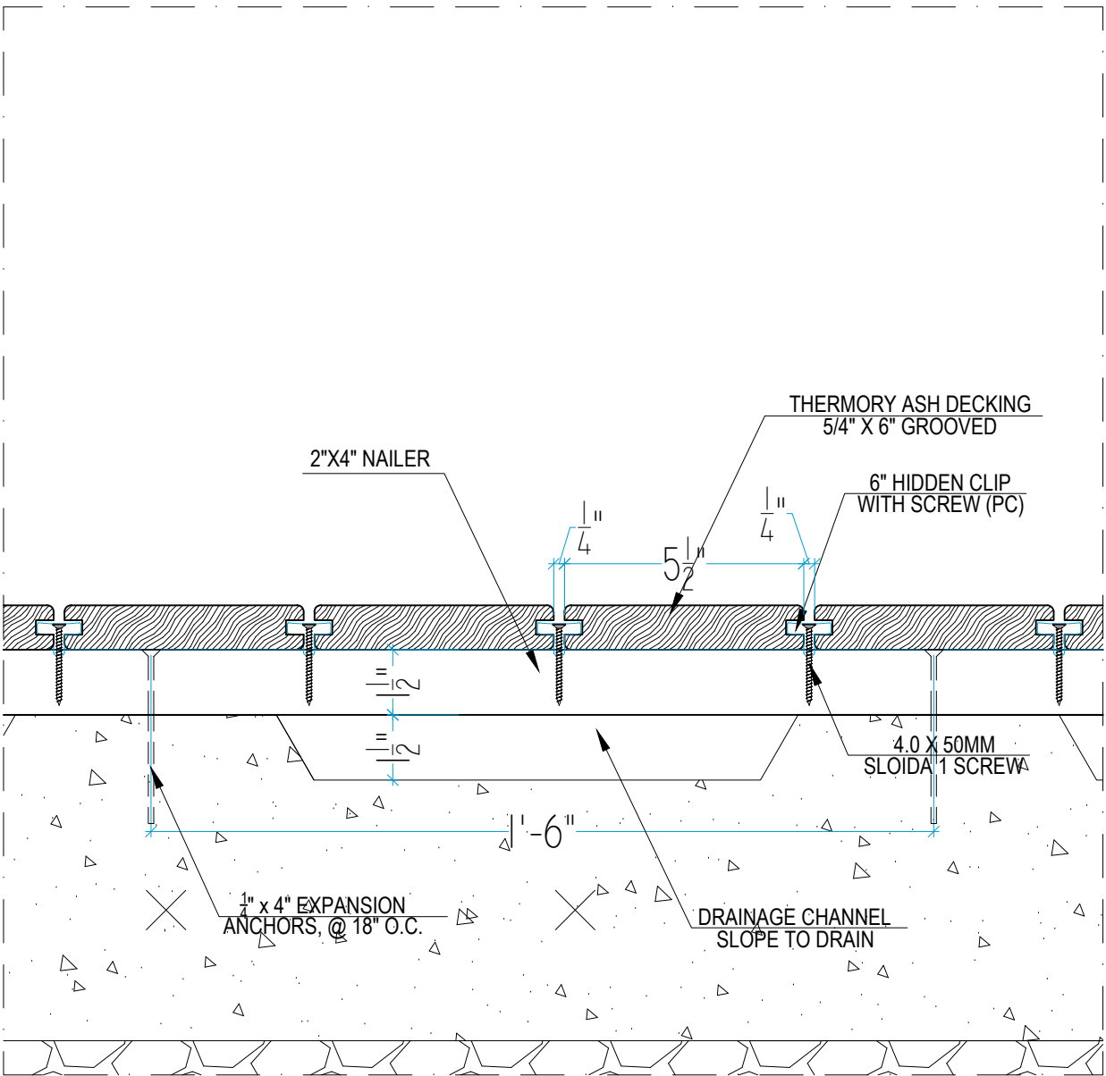
24 WOOD DECKING AT CONCRETE SLAB 3" = 1'-0"
