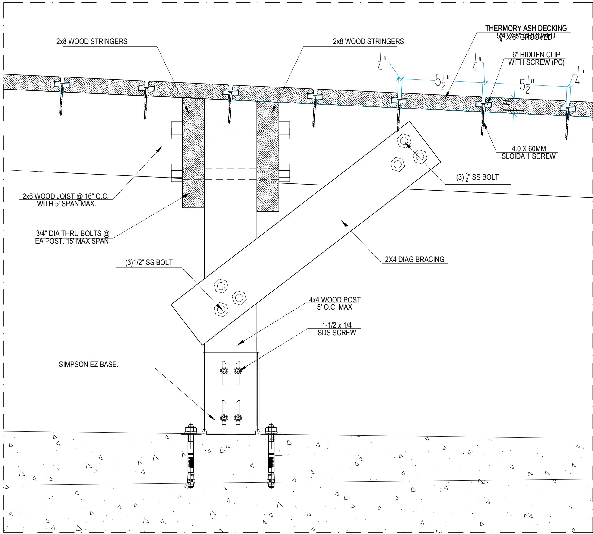
04 WOOD DECKING ON STRUCTURE
