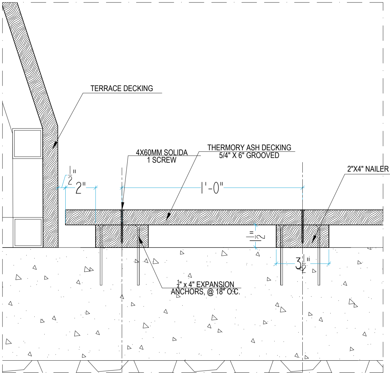
23 WOOD DECKING ON GRADE TO TERRACE 3" = 1'-0"
