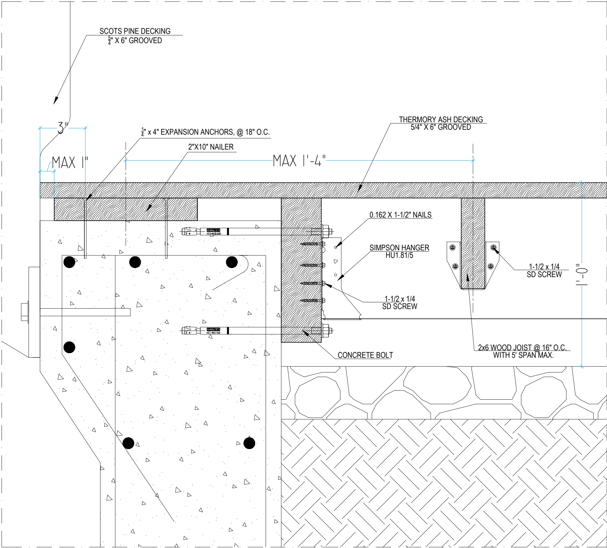
11 STEAM WALL ON GRADE 3" = 1'-0"
