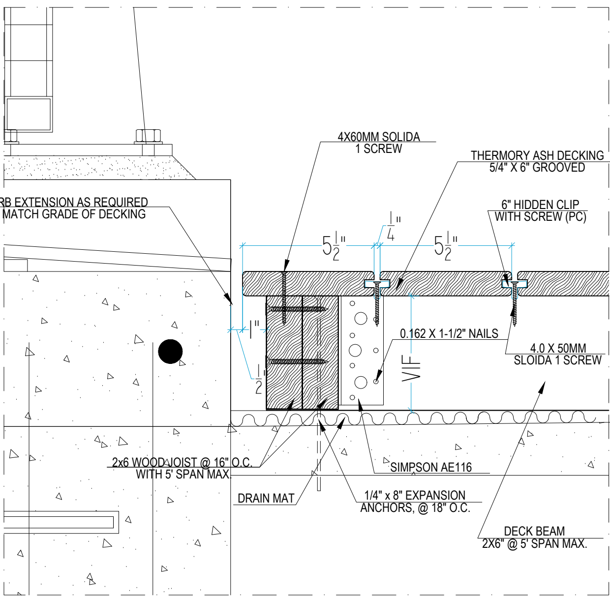
29 DIRECT MOUNT DECKING 3" = 1'-0"
