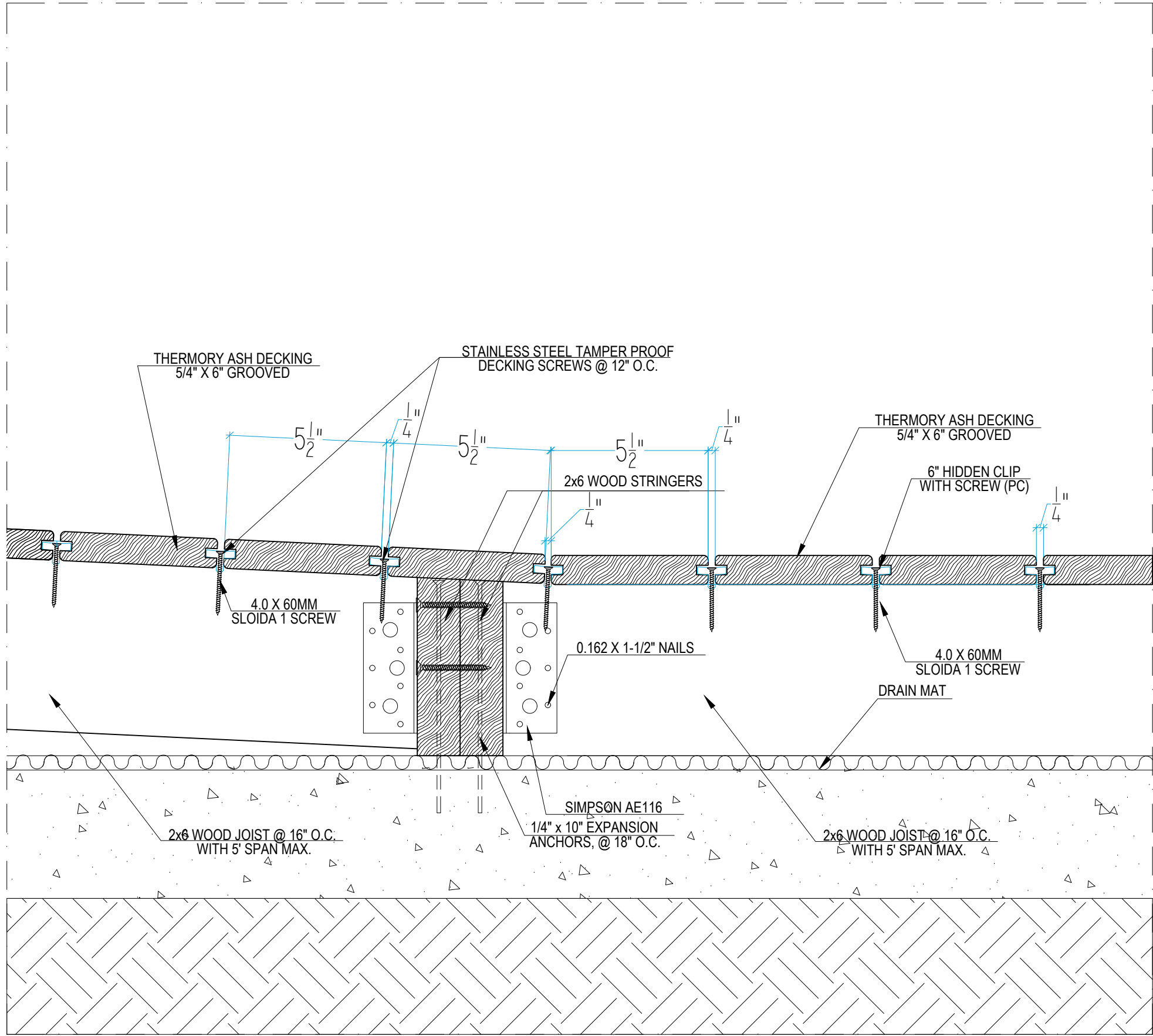
12 DIRECT MOUNT DECKING TO STRUCTURE 3" = 1'-0"
