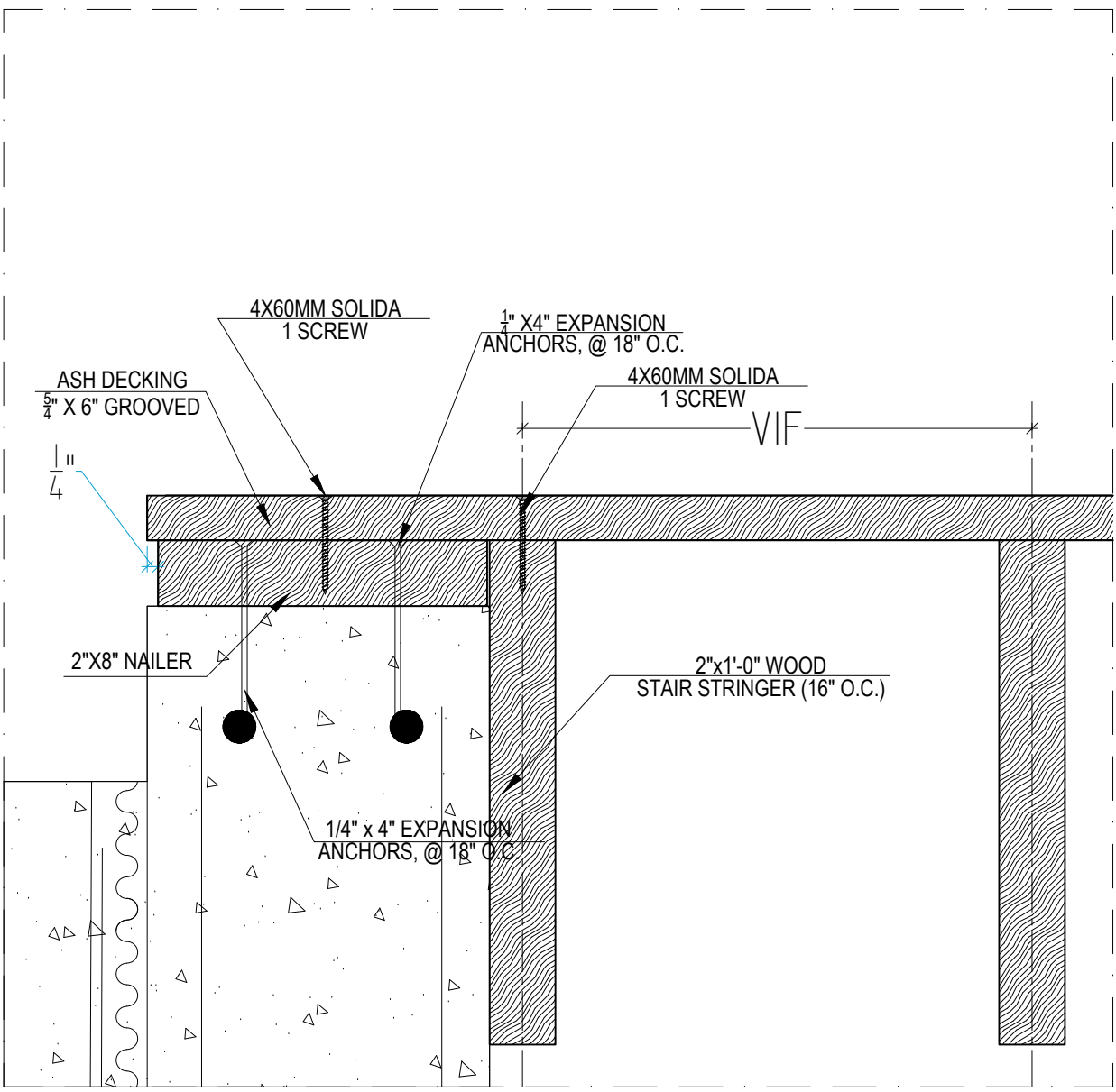
27 WOOD STAIR AT STEAM WALL 3" = 1'-0"
