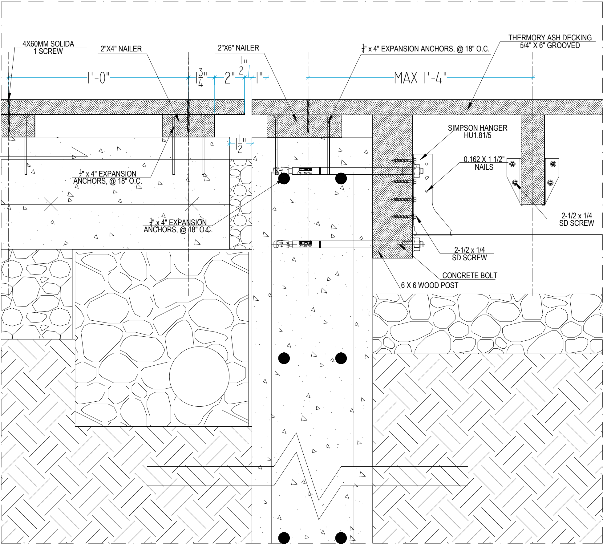
07 DECKING AT CONC. SLAB DRAINAGE 3" = 1'-0"
