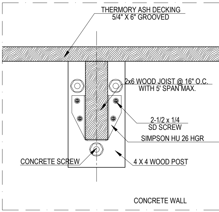
19 TYPICAL JOIST CONNECTION 3" = 1'-0"
