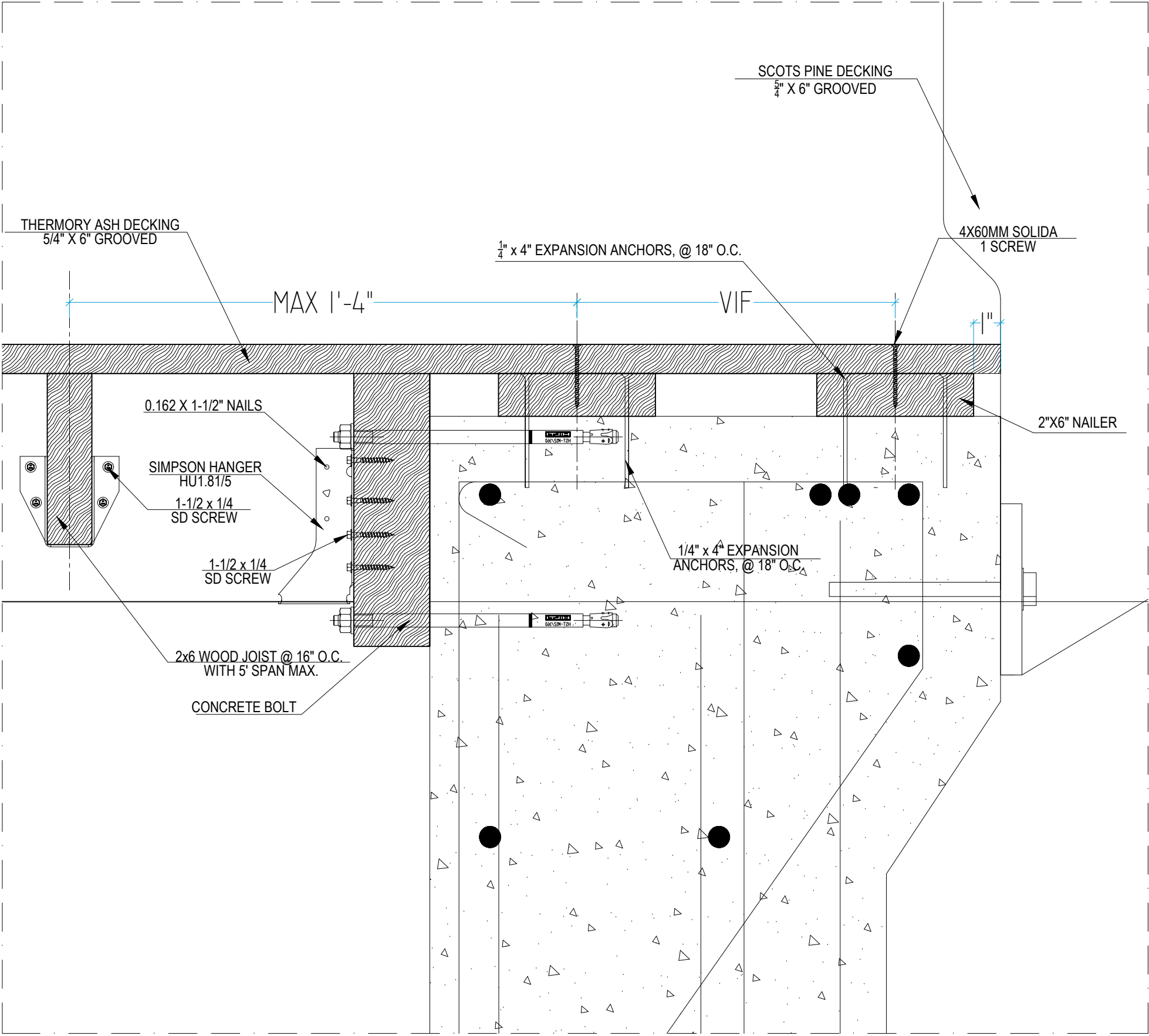
10 STEAM WALL AT DECKING 3" = 1'-0"
