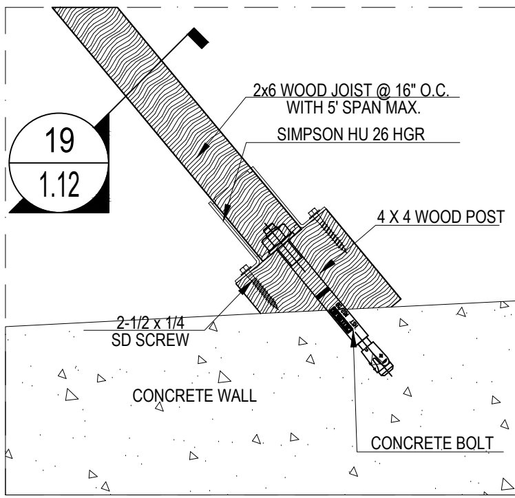
18 TYPICAL JOIST CONNECTION 3" = 1'-0"
